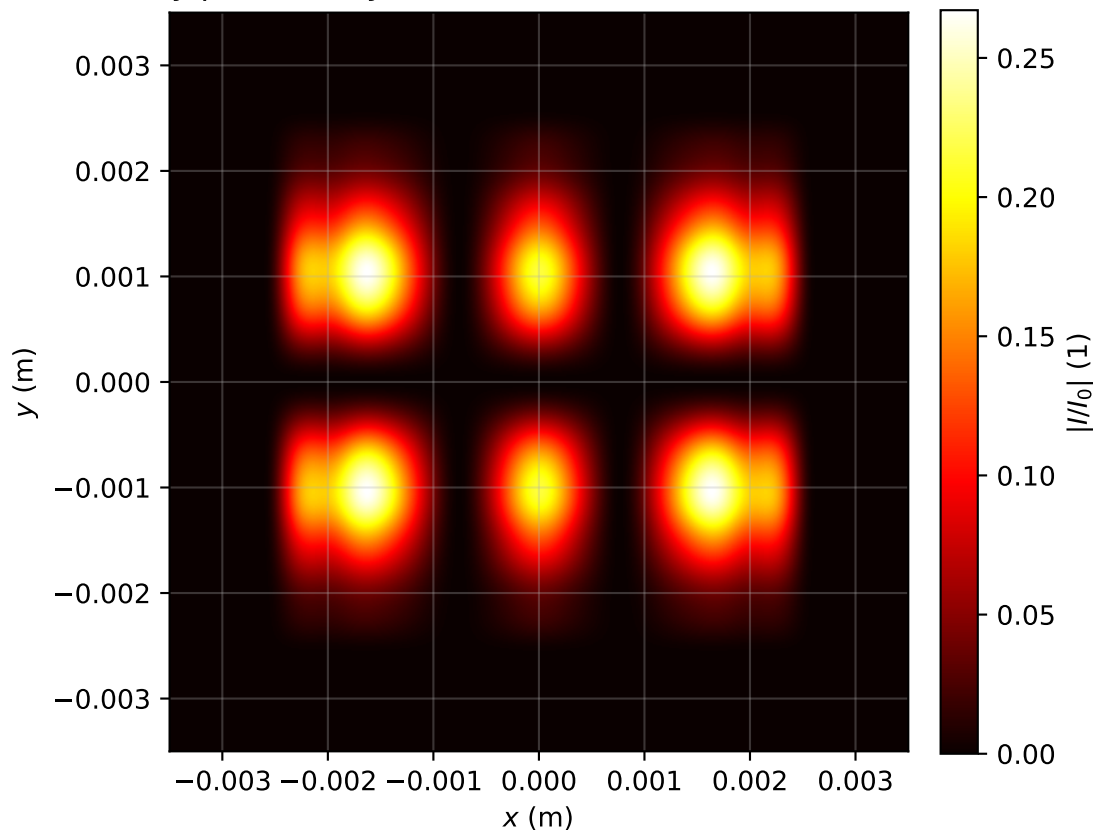
Intensity profile I(x, y, z = 3.742)/I_0 , P_{in}=1.0P_{cr} , artificial time
